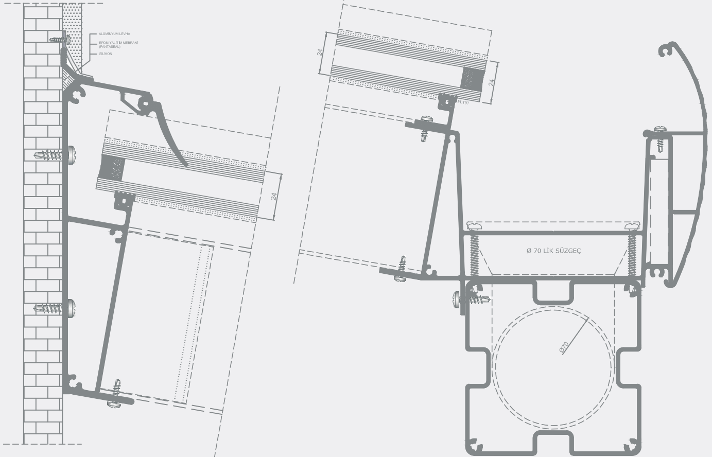
FC50-162 OLUK KAPAK GUTTER COVER
