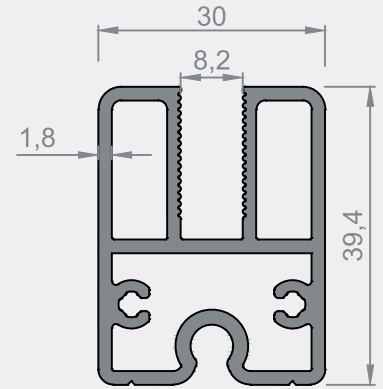
5710 - 1,056 kg/m
