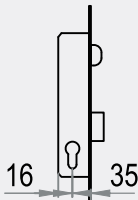
AKS14-M MAKARALI KİLİT MOURTISE LOCK WITH ROLLER
