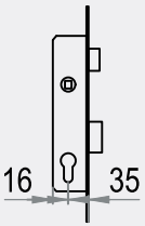
AKS14 DİLLİ KİLİT MOURTISE LOCK WITH CYLINDER
