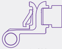
AKS06 PVC KANALLI MENTEŞE PVC CHANNEL HINGE
