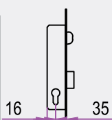
AKS14-M MAKARALI KİLİT MORTISE LOCK WITH ROLLER
