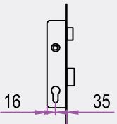
AKS14 DİLLİ KİLİT MORTISE LOCK WITH CYLINDER
