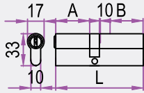
AKS10 BAREL CYLINDER
