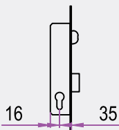
AKS14-M MAKARALI KİLİT MOURTISE LOCK WITH ROLLER
