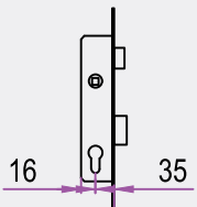
AKS14 DİLLİ KİLİT MOURTISE LOCK WITH CYLINDER
