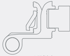
AKS06 PVC KANALLI MENTEŞE PVC CHANNEL HINGE
