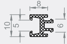
B7193 GAGA UZATMA PLASTİĞİ BEAK EXTENSION PLASTIC ( 6 M )
