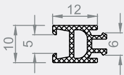
B7192 GAGA UZATMA PLASTİĞİ BEAK EXTENSION PLASTIC ( 6 M )
