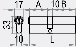
AKS10 BAREL CYLINDER
