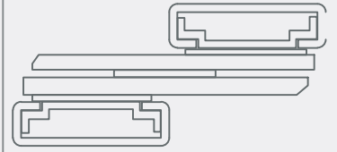
AKS21-XX PARALEL AÇILIM MAKAS PARALEL TOP-HUNG WINDOW
